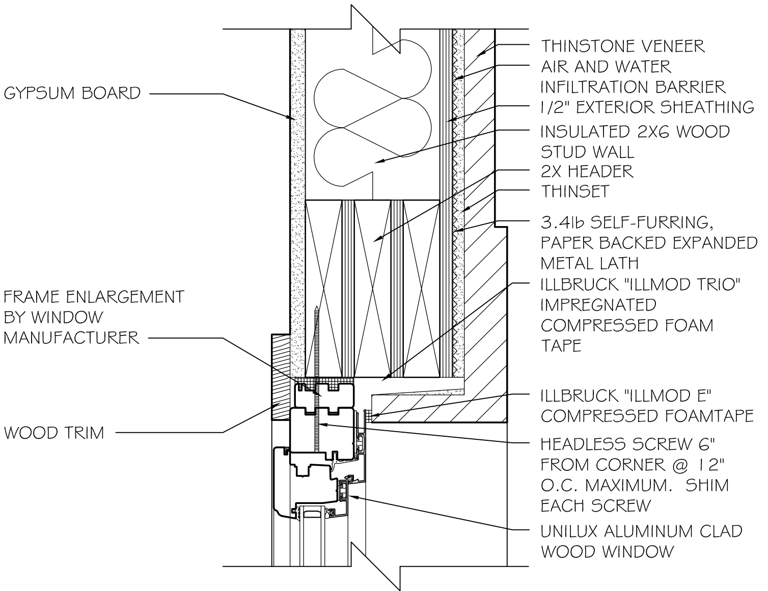
INBOUND HEAD DETAIL SCALE: 3" = 1'-0"
