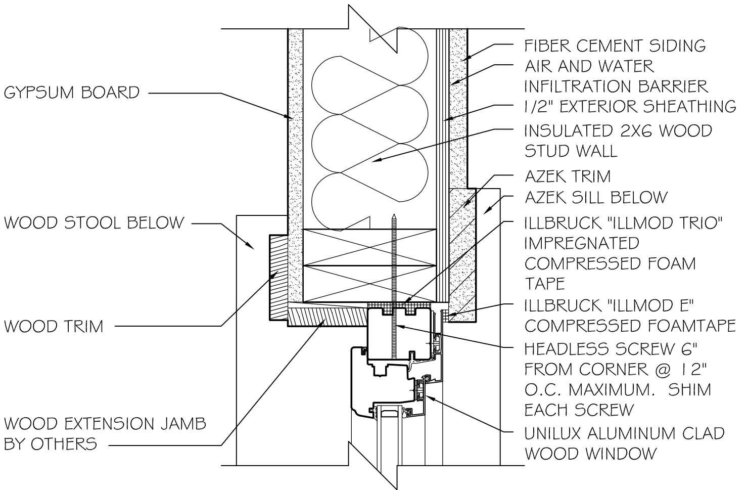
OUTBOUND JAMB DETAIL SCALE: 3" = 1'-0"
