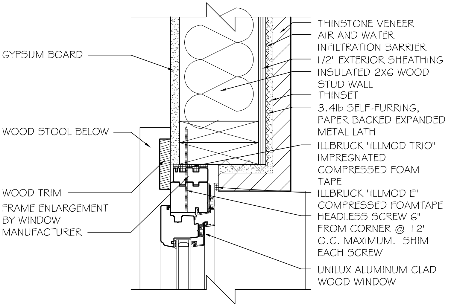
INBOUND JAMB DETAIL SCALE: 3" = 1'-0"
