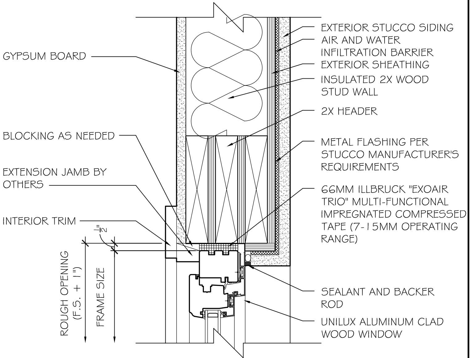
MIDBOUND HEAD DETAIL SCALE: 3" = 1'-0"
