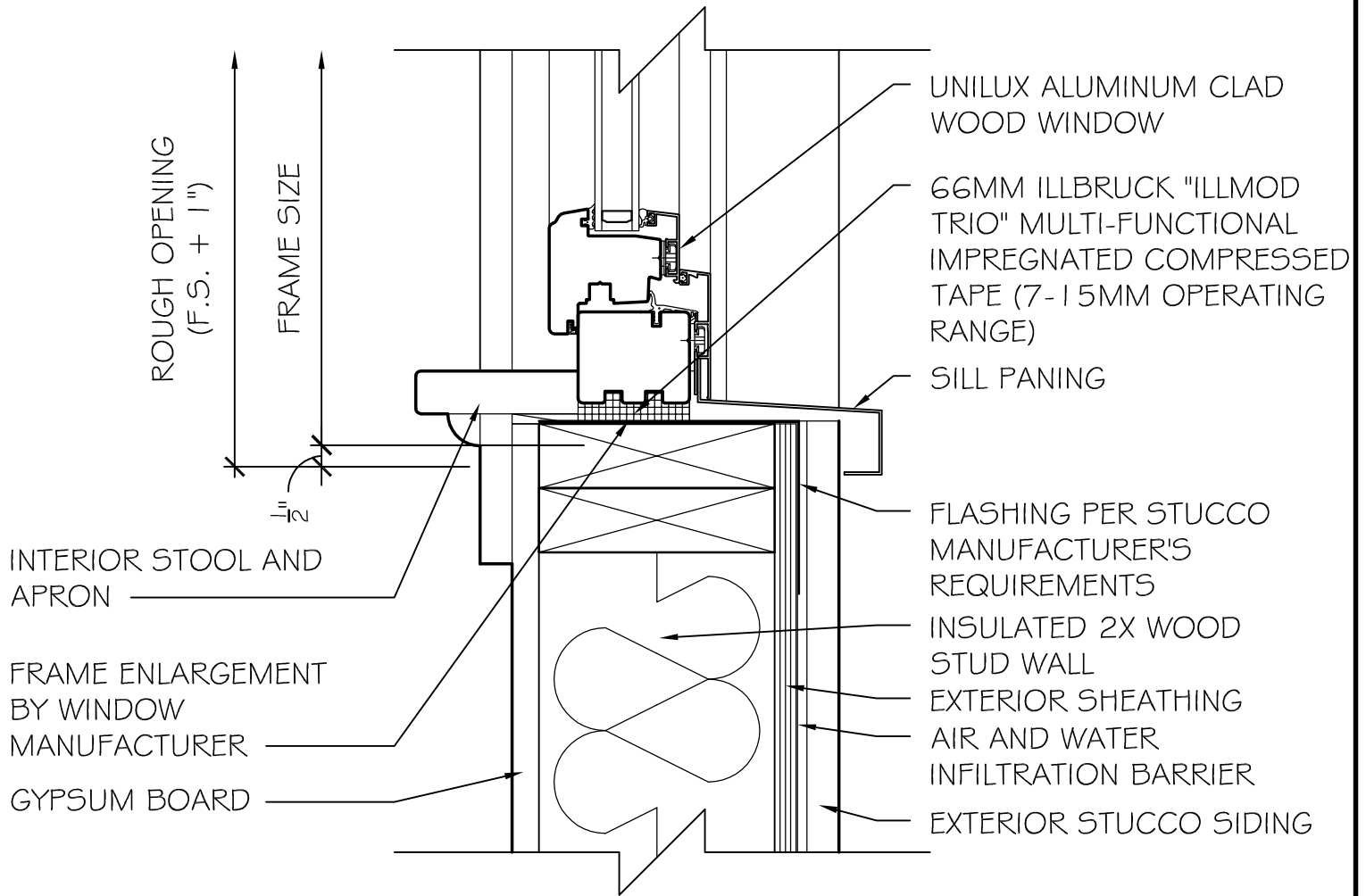
MIDBOUND SILL DETAIL SCALE: 3" = 1'-0"
